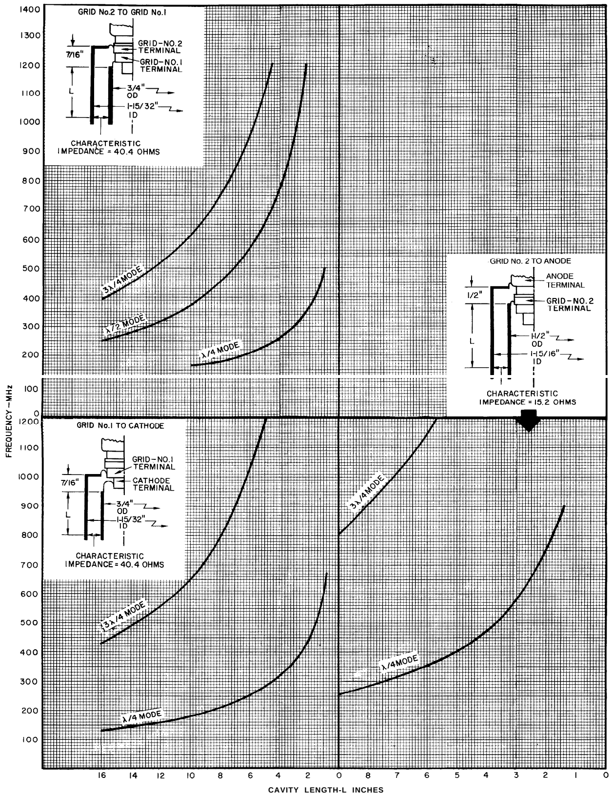
Figure 4 - Tuning Characteristics
