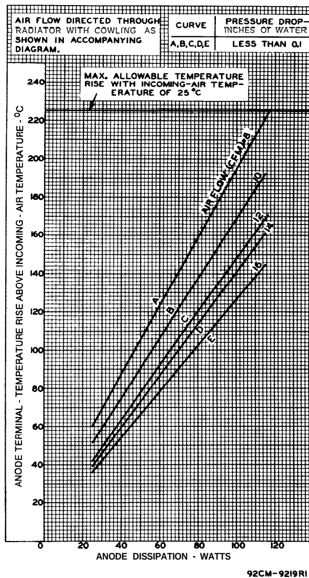
Figure 9 - Typical Cooling Requirements
