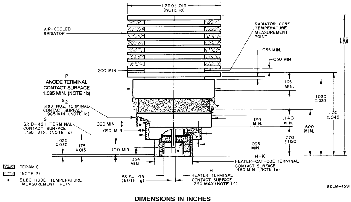
Figure 1 - Dimensional Outline
